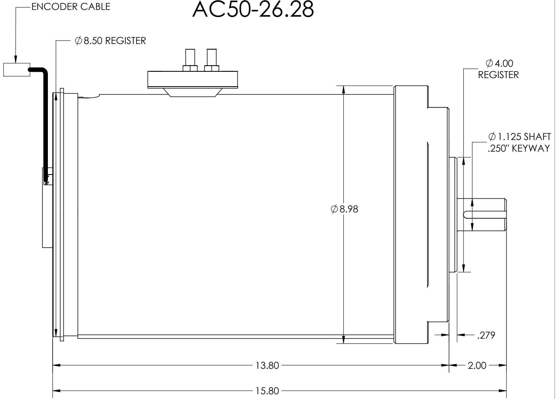
SIDE VIEW
